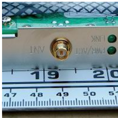
Female RP-SMA
